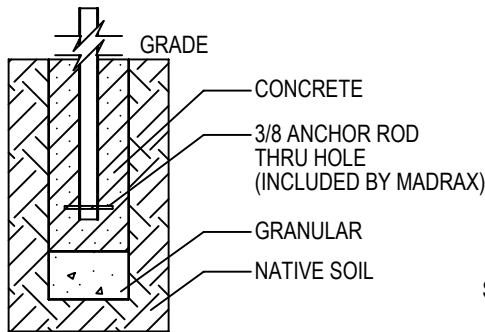
□ IN GROUND MOUNT (IG)
