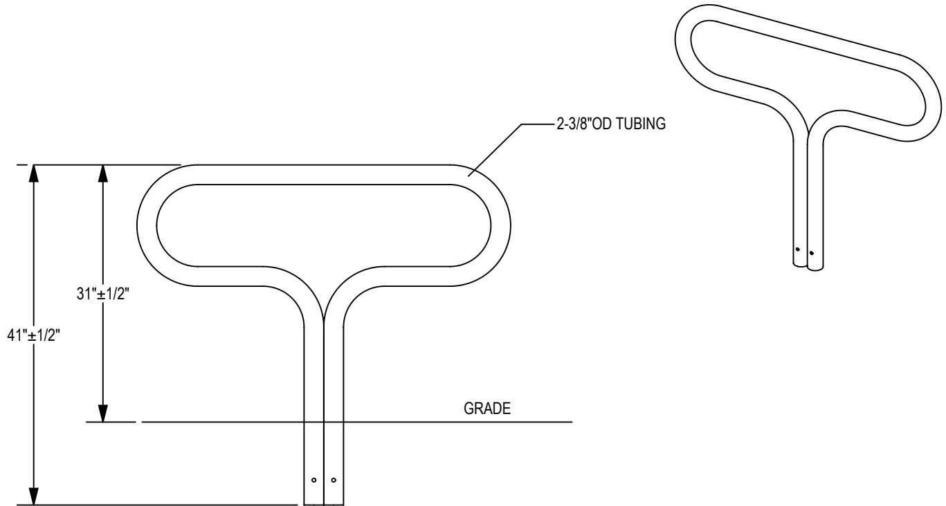
ELEVATION VIEW
