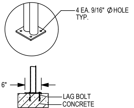
□ SURFACE FLANGE MOUNT (SF)
