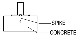
SURFACE FLANGE MOUNT (SF)
