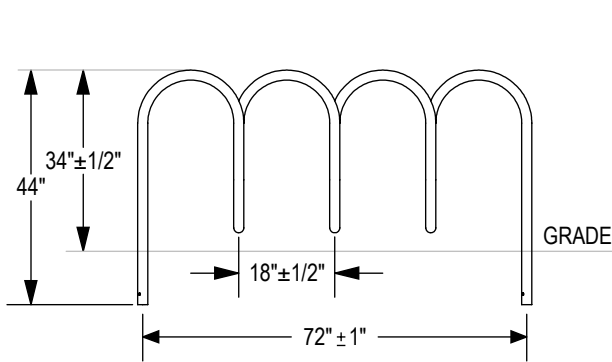
ELEVATION VIEWS
