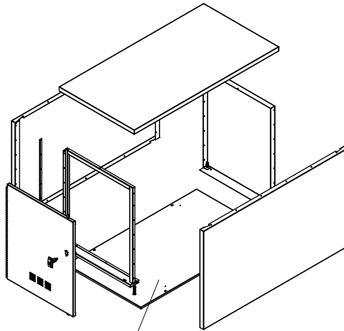
EXPLODED COMPONENT VIEW
