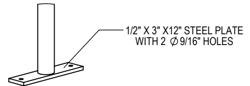
□ SURFACE FLANGE MOUNT (SF)
