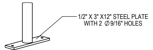
SURFACE FLANGE MOUNT (SF)
