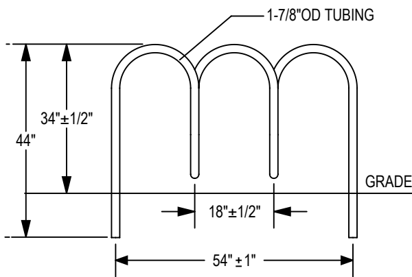
ELEVATION VIEWS 3 HOOP - 6 BIKE CAPACITY
